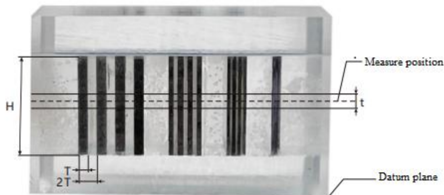
Figure A.2 Front View of Wire Pair Card
