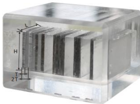
Figure A. 1 Three-dimensional structure of the line pair card
