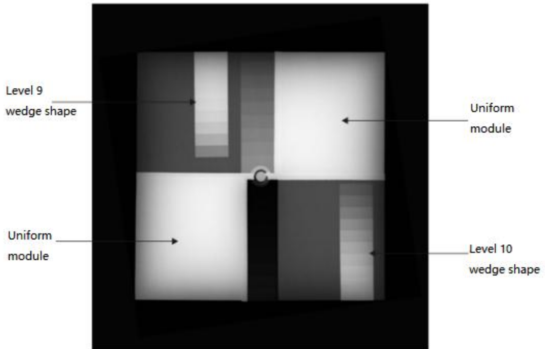
Figure A.1 TO J3 Radiographic Examination
