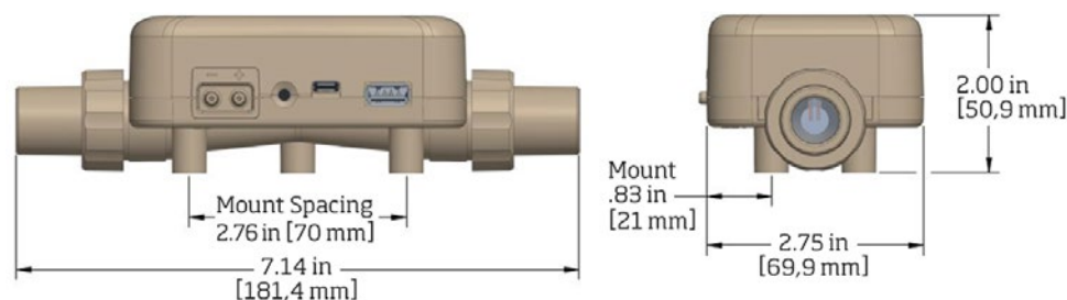
5300 Series Dimensions
